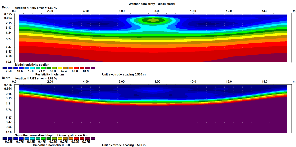
Figure 51. Example DOI plot for the beta.dat file. The top section shows the inverse resistivity model where the second reference model was used. As such, the inverse model values tend to be higher towards the bottom of the section as it trends to the reference resistivity used. The second section is the DOI section plot. If a DOI contour value of 0.1 is used as the cutoff point, the maximum depth of investigation in the middle of the survey line is about 3.5 meters. This DOI contour line becomes gradually shallower towards the ends of the line where there is less data.
