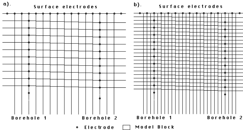
Figure 11. Arrangement of the electrodes in a cross-borehole survey. (a) The default standard model where the dimensions of the model blocks are equal to the spacing between the electrodes. (b) An alternative model with finer blocks with dimensions about half the spacing between the electrodes.
