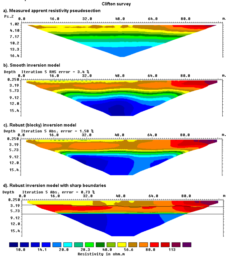
Figure 19. Models for the Clifton survey from the different inversion methods are shown together. Note the boundary between the high resistivity sand layer and the underlying low resistivity clay layer is much better resolved in the blocky and sharp boundary inversion methods.
