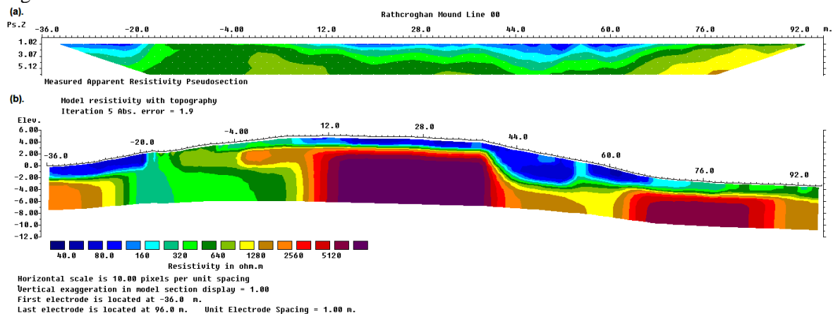
Figure 37. Example of the model for the Rathcroghan Mound data set. (a) Measured apparent resistivity pseudosection. (b) Inverse model section with topography.
