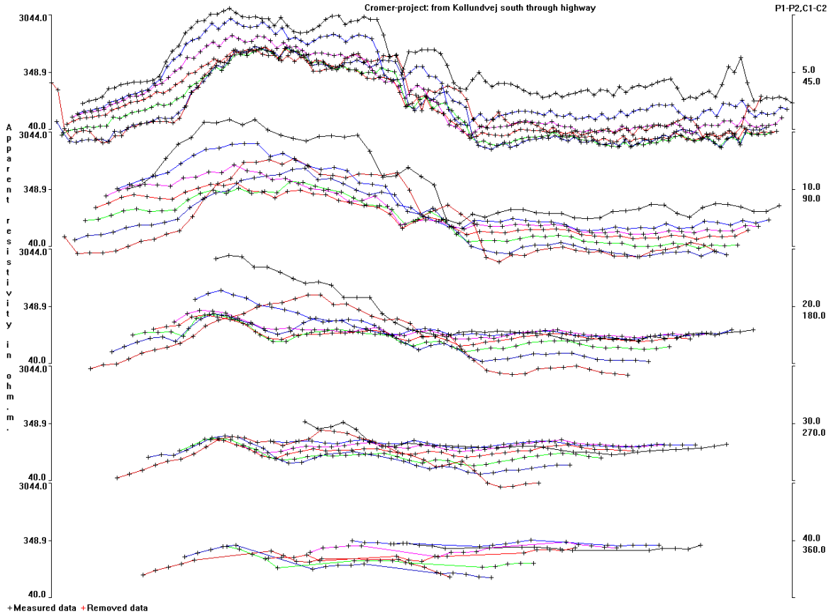
Figure 27. Plot of a CROMER2.DAT multiple gradient array data set in the form of profiles using the approximate pseudodepth method.
