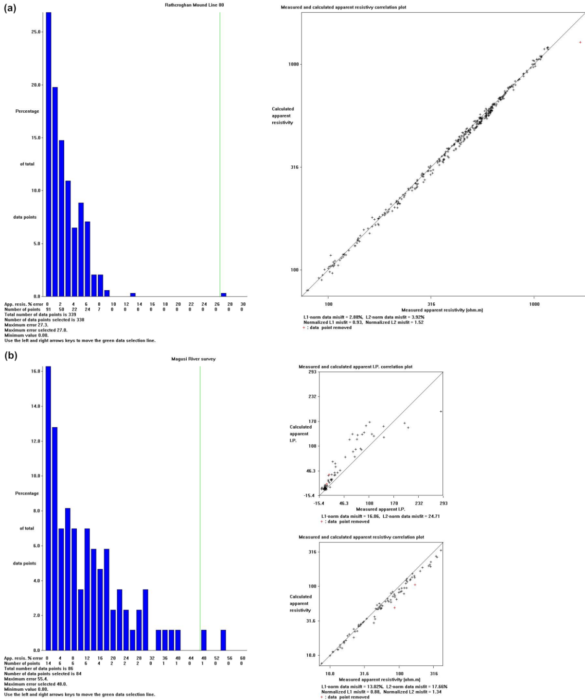
Figure 43. Histogram and scatter plots for the inversion results of the (a) RATHCRO.DAT and (b) IPMAGUSI.DAT data sets.
